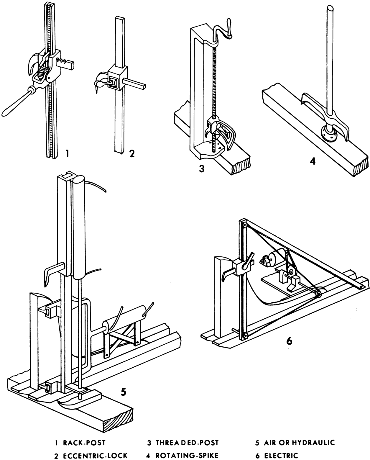
Figure 8-12. Fixed-post types of manually operated dogs.
